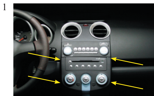
Remove the dashboard panel at the location of the arrows.
