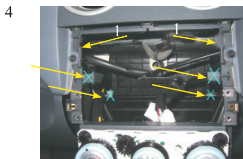
Remove the original plastic mounting frame at the location of the arrow/ cross.
