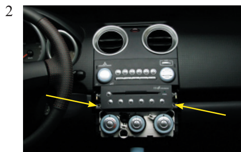
Remove the CD player. This is tighten by two screws
