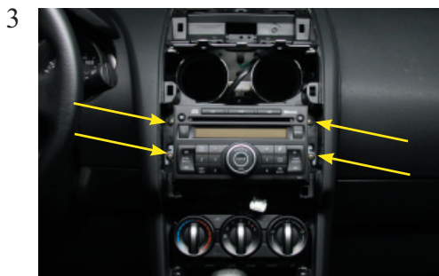
Remove the four screws at the location of the arrows. Remove the radio.
